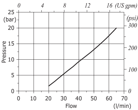
VDFR 100-150 pressure drop vs. flow (E→U1-U2) and (U1-U2→E)
